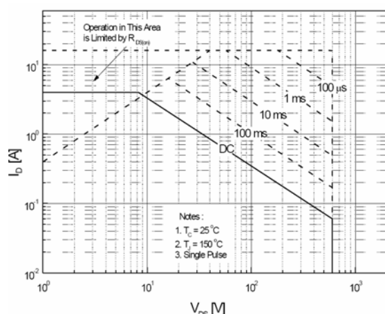
Maximum Safe Operating Area For JCS4N60FB
