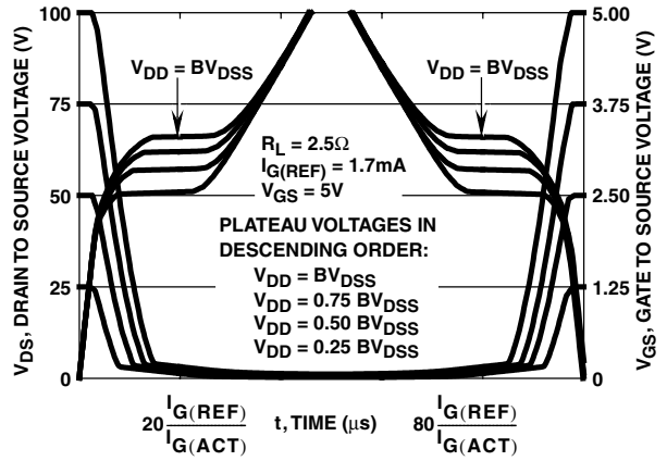
FIGURE 15. SWITCHING WAVEFORMS FOR CONSTANT GATE CURRENT
