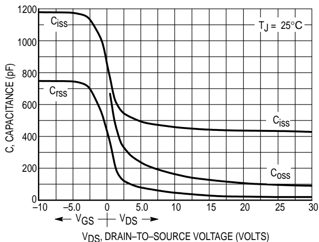
Figure 8. Capacitance Variation
