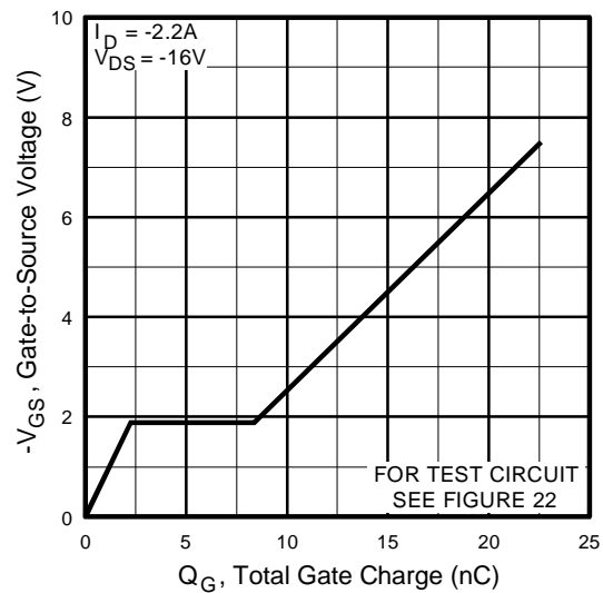
Fig 17. Typical Gate Charge Vs. Gate-to-Source Voltage
