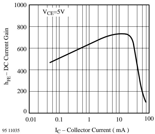
95 11035 h_{FE} – DC Current Gain Figure 18. DC Current Gain vs. Collector Current
