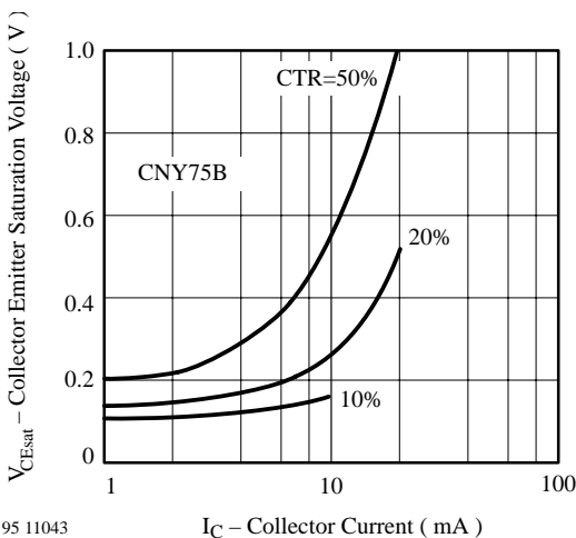
95 11043 V_{CESat} – Collector Emitter Saturation Voltage ( V ) Figure 16. Coll. Emitter Sat. Voltage vs. Coll. Current
