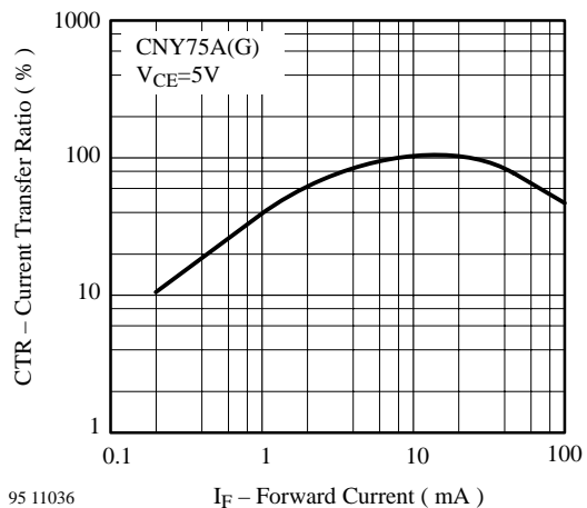
95 11036 CTR – Current Transfer Ratio ( % ) Figure 19. Current Transfer Ratio vs. Forward Current
