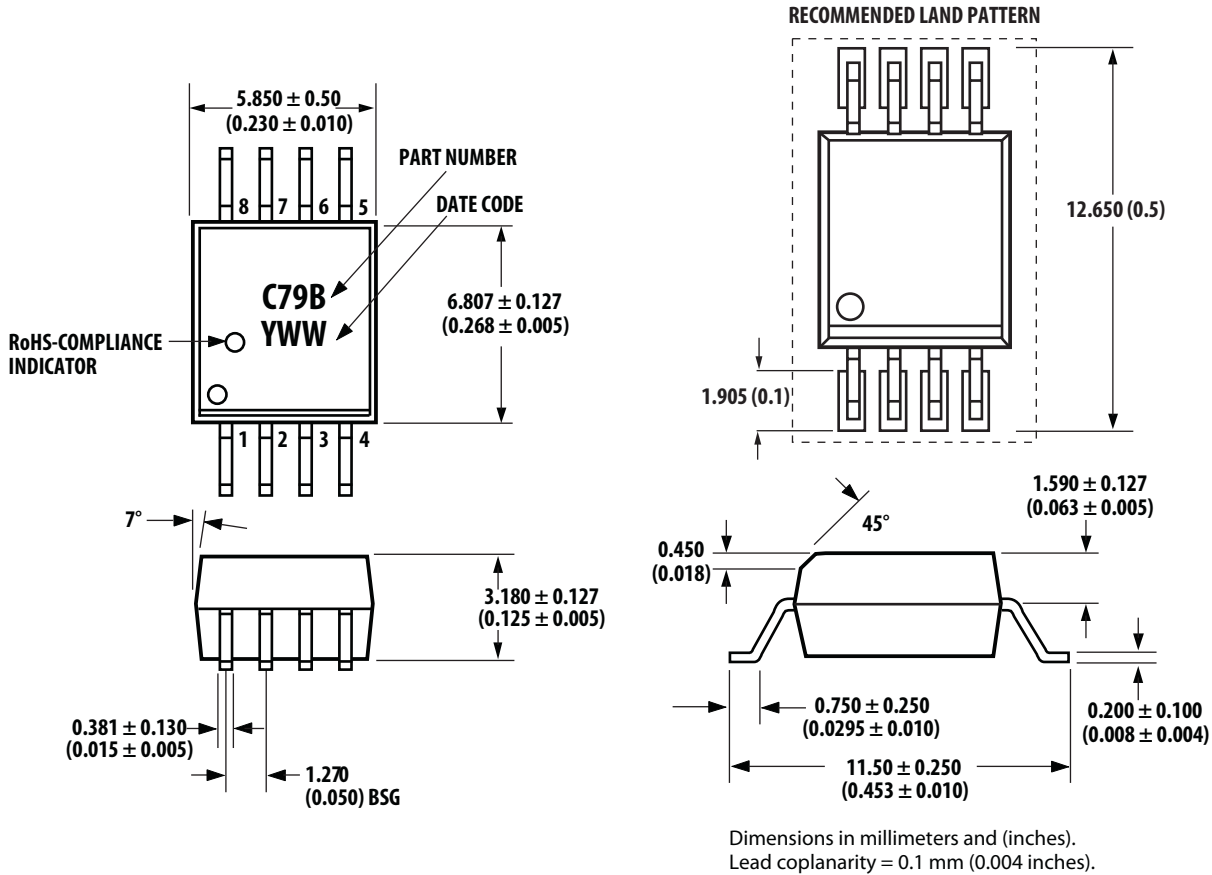
Figure 2. SSO-8 package.
