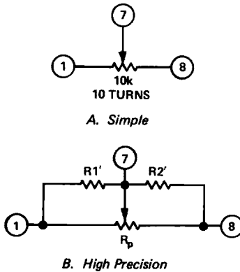
Figure 1. Nulling Circuits
