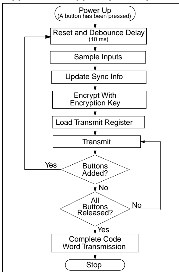
FIGURE 2-2: ENCODER OPERATION
