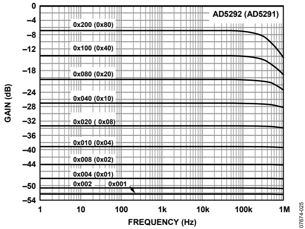
Figure 25. 20 kΩ Gain vs. Frequency vs. Code (AD5292)
