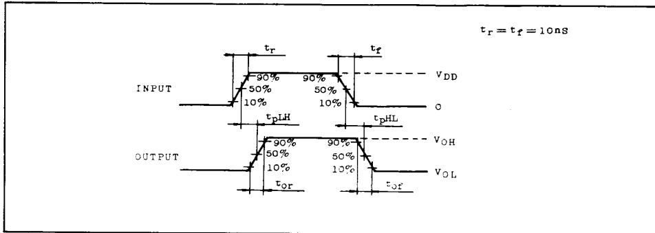
t_{pd} - V_{DD}
