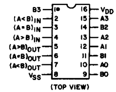
TERMINAL ASSIGNMENT
