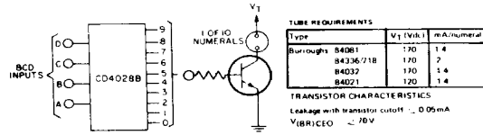
Fig. 14 — Neon readout (Nixie Tube ▲ ) display application.
