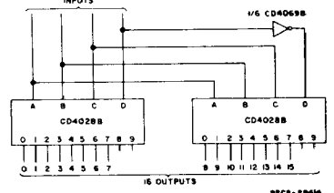
Fig. 13 — Code conversion circuit.
