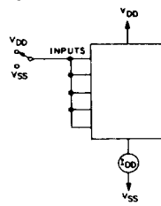
Fig. 12 — Quiescent device current test circuit.
